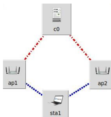
Gambar 1. Bicasting Network Topologi
