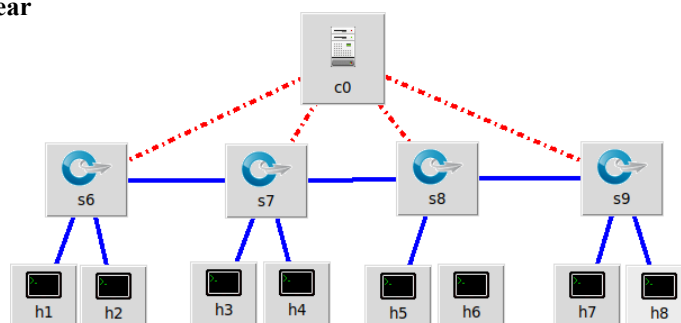
Gambar 3. Topologi Linear
